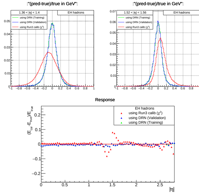
FIGURE 4.23: 1D-energy response distributions of EH hadrons (on top) for different \eta bins and inclusive in E_t . Average energy response (bottom) after using \chi^2 (red), DRN (blue & green) calibration methods, as a function of |\eta| for EH hadrons.
