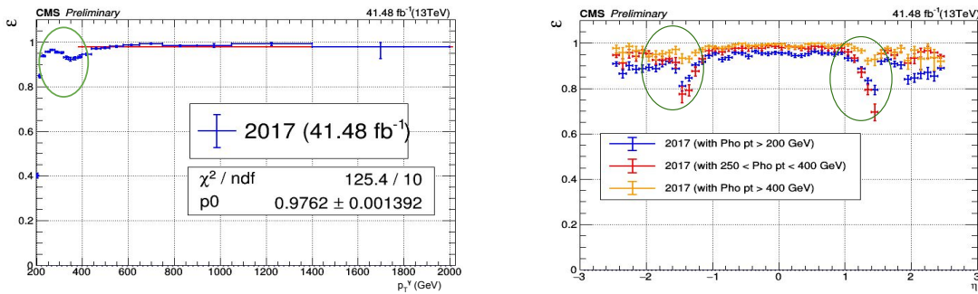
FIGURE 5.6: The photon trigger efficiencies ( \epsilon ) wrt transverse momenta of photon ( p_T^\gamma ) (left) and pseudorapidity of photon ( \eta ). Green circles shows kinks in trigger efficiencies for both left and right figures.
