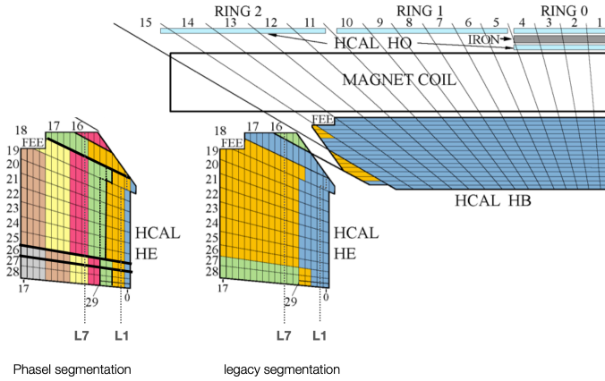
FIGURE 3.7: A longitudinal view ( r - z plane) showing HCAL detector during the 2016 LHC Run 2 (right) and phase 1 segmentation of the HE (left) which is upgraded during the 2018 LHC Run 2. The numbers on top and on left refer to the tower numbers. The numbers on the bottom (0–17) indicate the scintillator layers numbers inserted into slots in the absorber [76].
