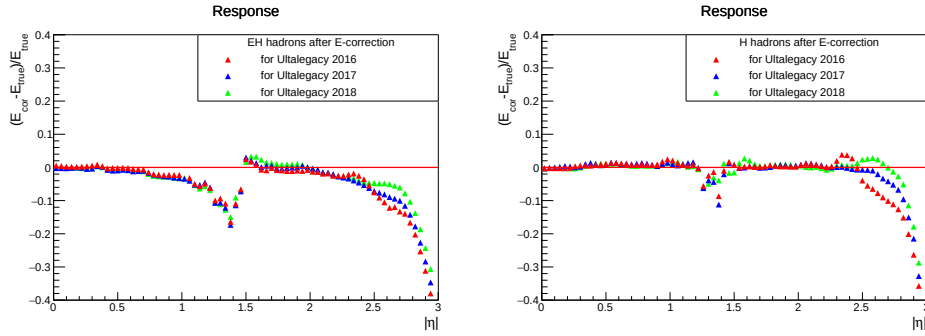
FIGURE 4.7: Average energy response after applying energy dependent calibrations as a function of |\eta| for EH hadrons(left) and H hadrons(right).
