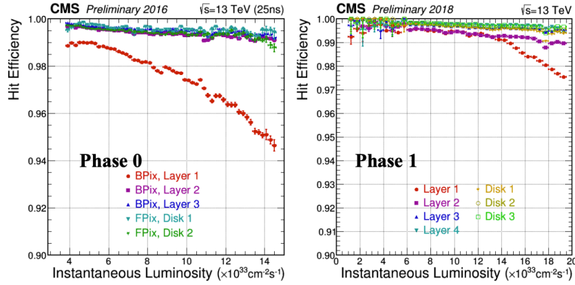
FIGURE 3.5: Hit efficiency over large range in luminosity for phase 0 (during 2016) and phase 1 (during 2018 upgrades) [75].
