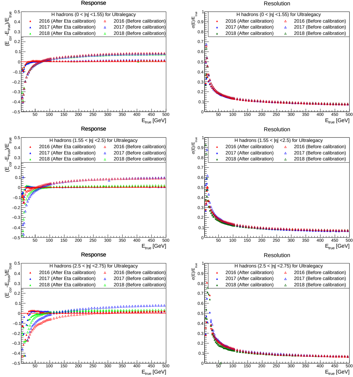
FIGURE 4.11: Final response (left column) & resolution (right column) of H hadrons obtained in the bins of E_t shown for barrel (row 1), endcap within tracker (row 2) and endcap outside tracker (row 3) for 2016, 2017, and 2018. The solid and empty symbols correspond to corrected and raw energy measurements respectively.
