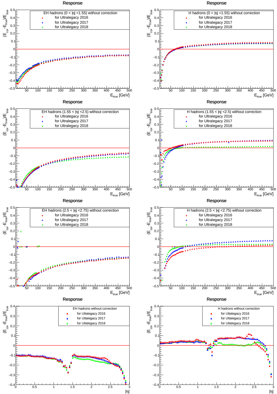
FIGURE 4.4: Average raw energy response i.e. (E_t - E_{\text{total}}^{\text{raw}})/E_t as a function of E_t (top) and |\eta| (bottom) for EH (left) and H (right) hadrons for Ultra legacy conditions corresponding to 2016, 2017 & 2018.
