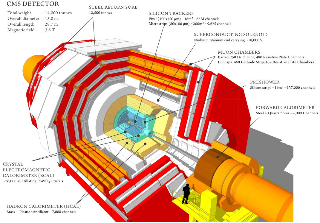
FIGURE 3.3: Sectional view of the CMS detector [69].
