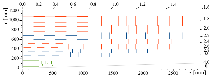
FIGURE 3.4: Schematic view for the first quadrant of the CMS tracker in r - z coordinates [72]. Layers with green color represents the inner pixel tracker and orange (blue) color means single (double) sided modules represents outer strip tracker. Single sided modules have only reverse p-n junction sensor whereas double sided modules have two silicon sensors mounted back to back [73].
