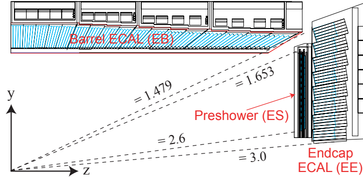
FIGURE 3.6: A schematic view showing only one quarter of the ECAL detector [70].
