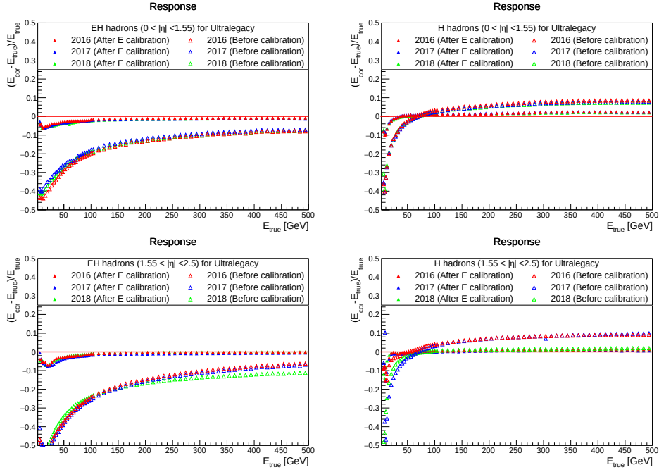
FIGURE 4.6: Average energy response after applying energy dependent calibrations as a function of E_t for EH hadrons(left) and for H hadrons(right).
