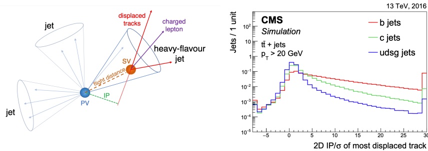
FIGURE 3.13: Pictorial representation of the secondary vertex in the heavy flavored jet (left) and 2D IP significance distribution of the most displaced track (right) for different jet flavours. [93]. 2D IP/\sigma plot shows the higher IP value for b-jets.
