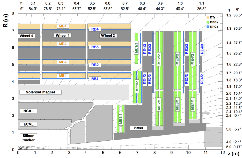
FIGURE 3.8: A schematic r-z view of the CMS detector showing muon system for Run 2 in details. It includes DTs (MB), CSCs (ME), and RPCs (RB or RE), which are described by respective colours in the legend. Here M denotes Muon, B stands for Barrel and E for Endcap [77].
