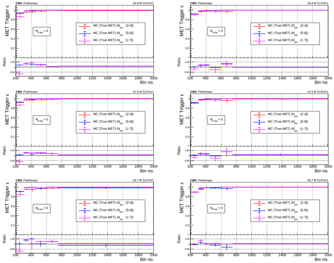
FIGURE C.2: MET trigger efficiency for different N_{b\text{-tags}} & N_{jets} combinations in same MET SR bins using MC background samples as a sum of W/tt/Z (source of true MET) only but not QCD & Gjets (Fake MET).
