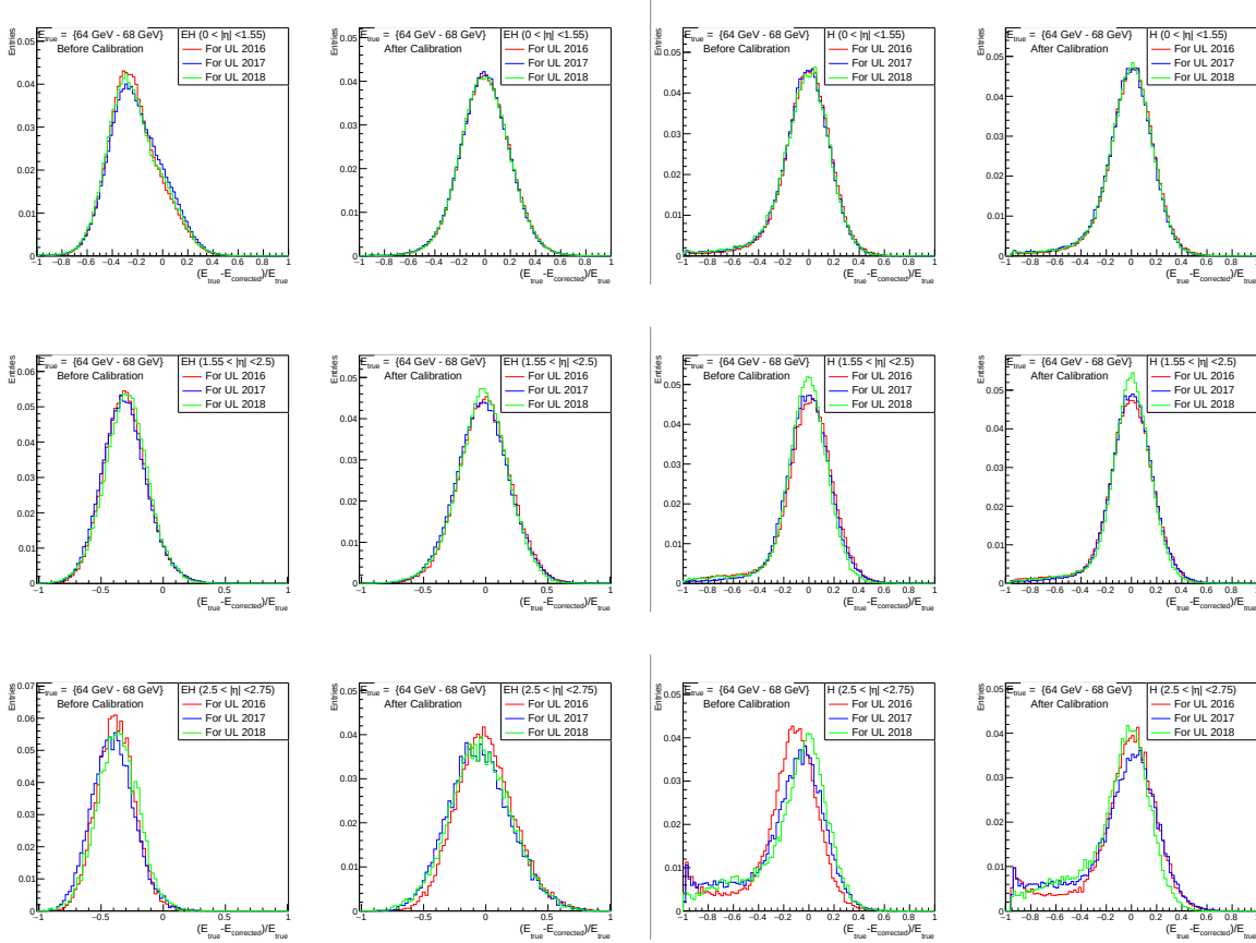
FIGURE 4.13: 1st (3rd) and 2nd (4th) columns represent 1D energy response distributions before and after final calibrations for EH (H) hadrons respectively. Top, middle and bottom rows represent the barrel, endcap within tracker and endcap outside tracker regions.
