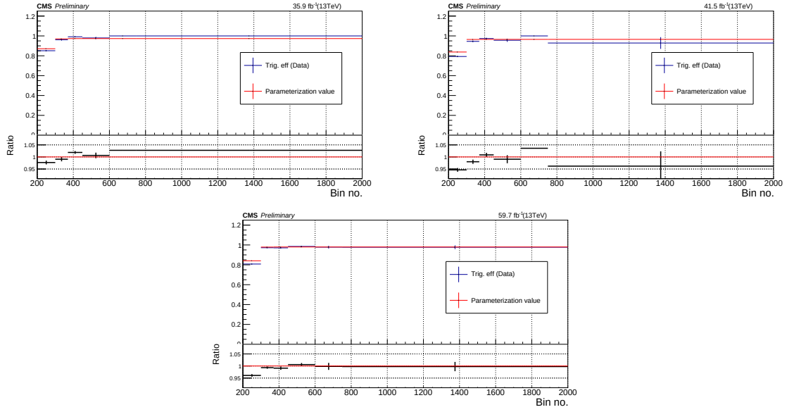
FIGURE C.1: Comparison of MET trigger efficiency from data and parameterization function
