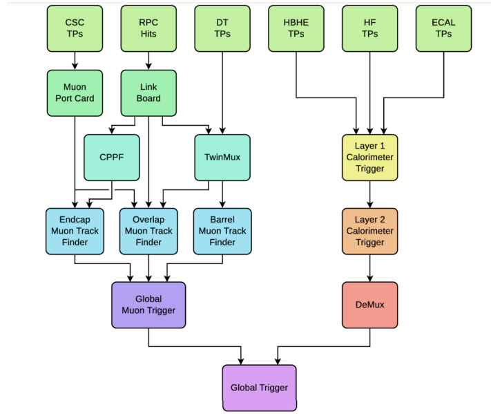
FIGURE 3.9: Overview of the CMS L1 trigger system for Run II [80].
