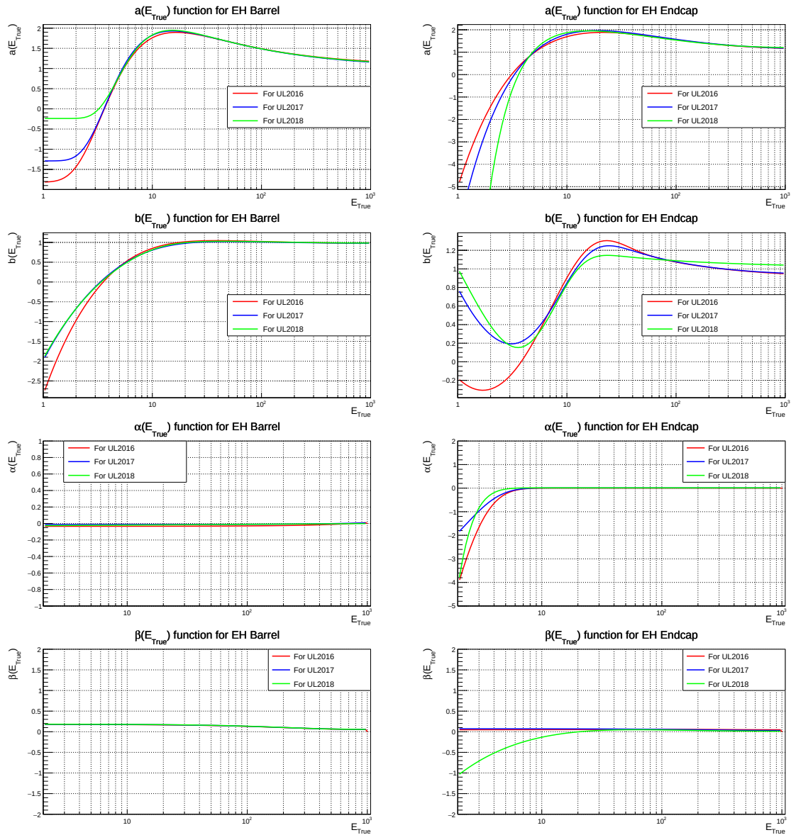
FIGURE 4.8: Calibration parameters for EH hadrons in barrel (left column) and endcap regions (right column): a(E_t) (row 1), b(E_t) (row 2), \alpha(E_t) (row 3) and \beta(E_t) (row 4).
