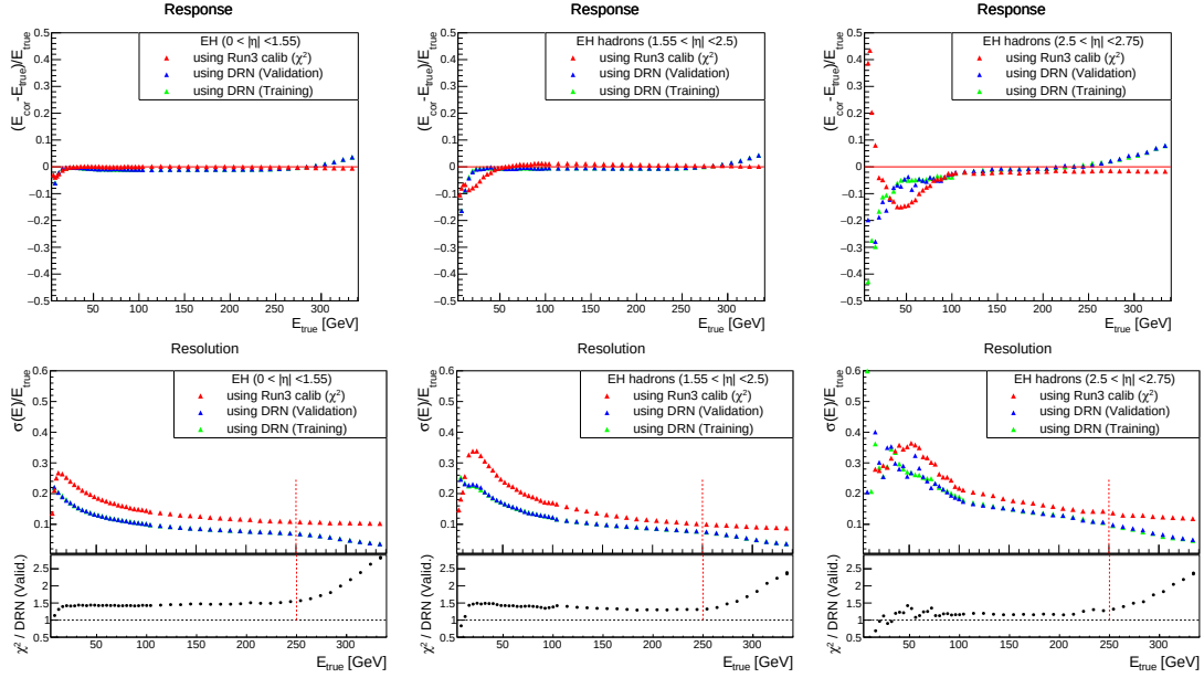
FIGURE 4.21: Average energy response (top) and resolution (bottom) after using \chi^2 (red), DRN (blue & green) calibration methods, as a function of E_t for EH hadrons. After red dashed line at E_t = 250 GeV, there is an edge effect and that can be ignored for now.
