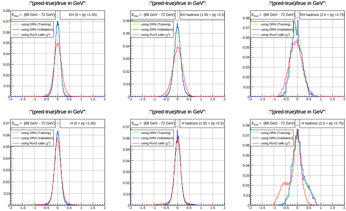
FIGURE 4.20: 1D energy response distribution after calibrations using \chi^2 (red), DRN (blue & green) calibrations for EH hadrons(top) and for H hadrons(bottom). These energy responses are in the E_t range of 68–72 GeV for various \eta regions.
