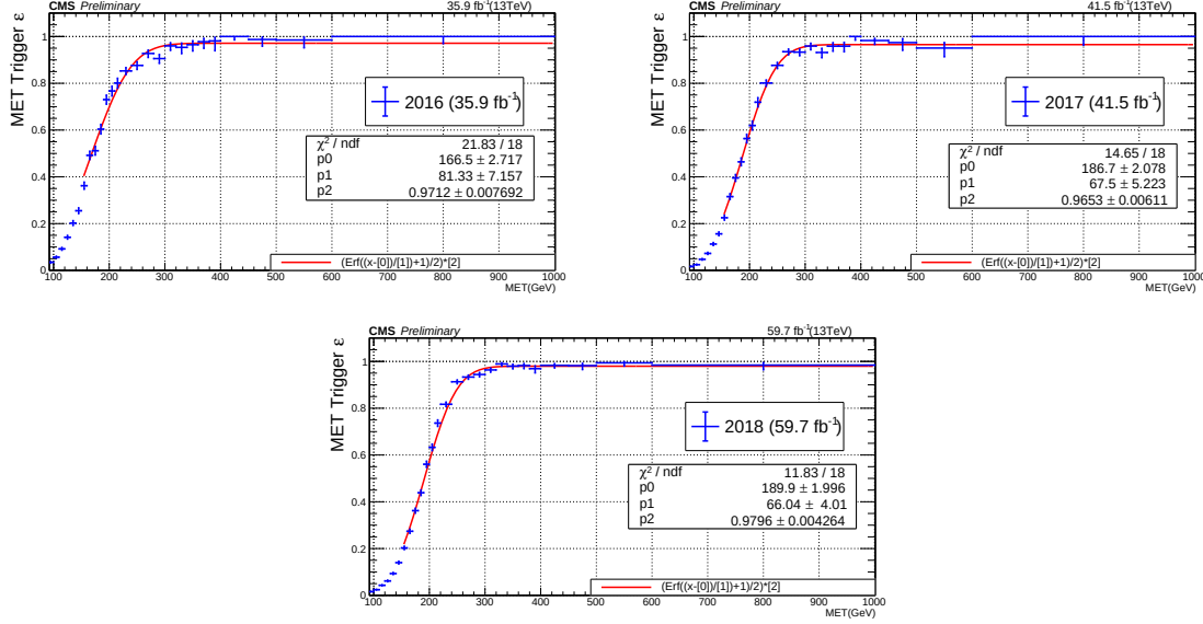
FIGURE 5.5: MET X MHT trigger efficiency, \epsilon_{MET} with respect to p_T^{\text{miss}} using single electron dataset for years 2016, 2017, 2018.
