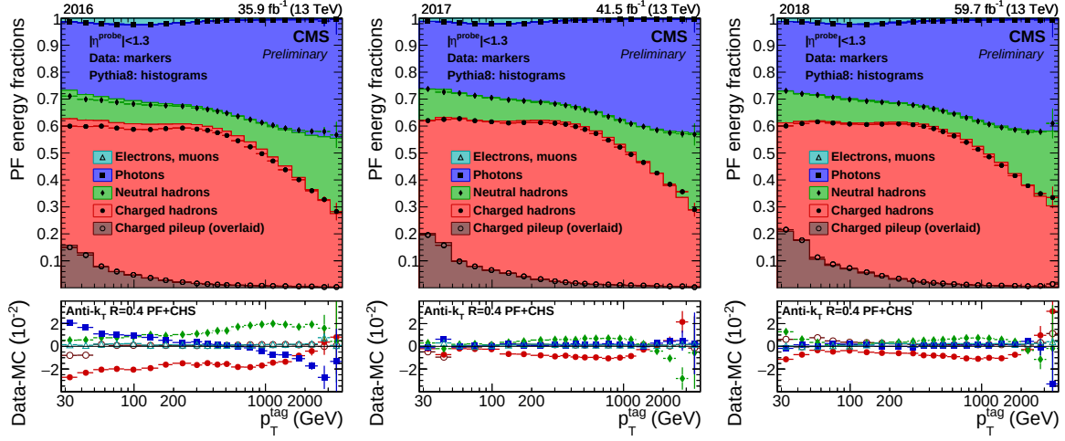
FIGURE 4.1: Comparisons of PF jet composition measured as a fraction of energy carried by PF photons, charged hadrons, neutral hadrons, and electrons and muons in data and MC simulation for 2016 (left), 2017 (middle), and 2018 (right) [96]
