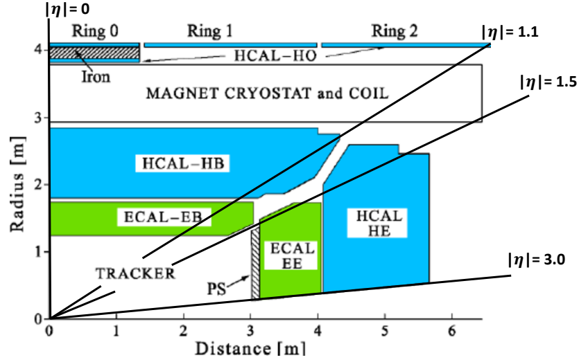
FIGURE 4.5: The CMS longitudinal layout [101].
