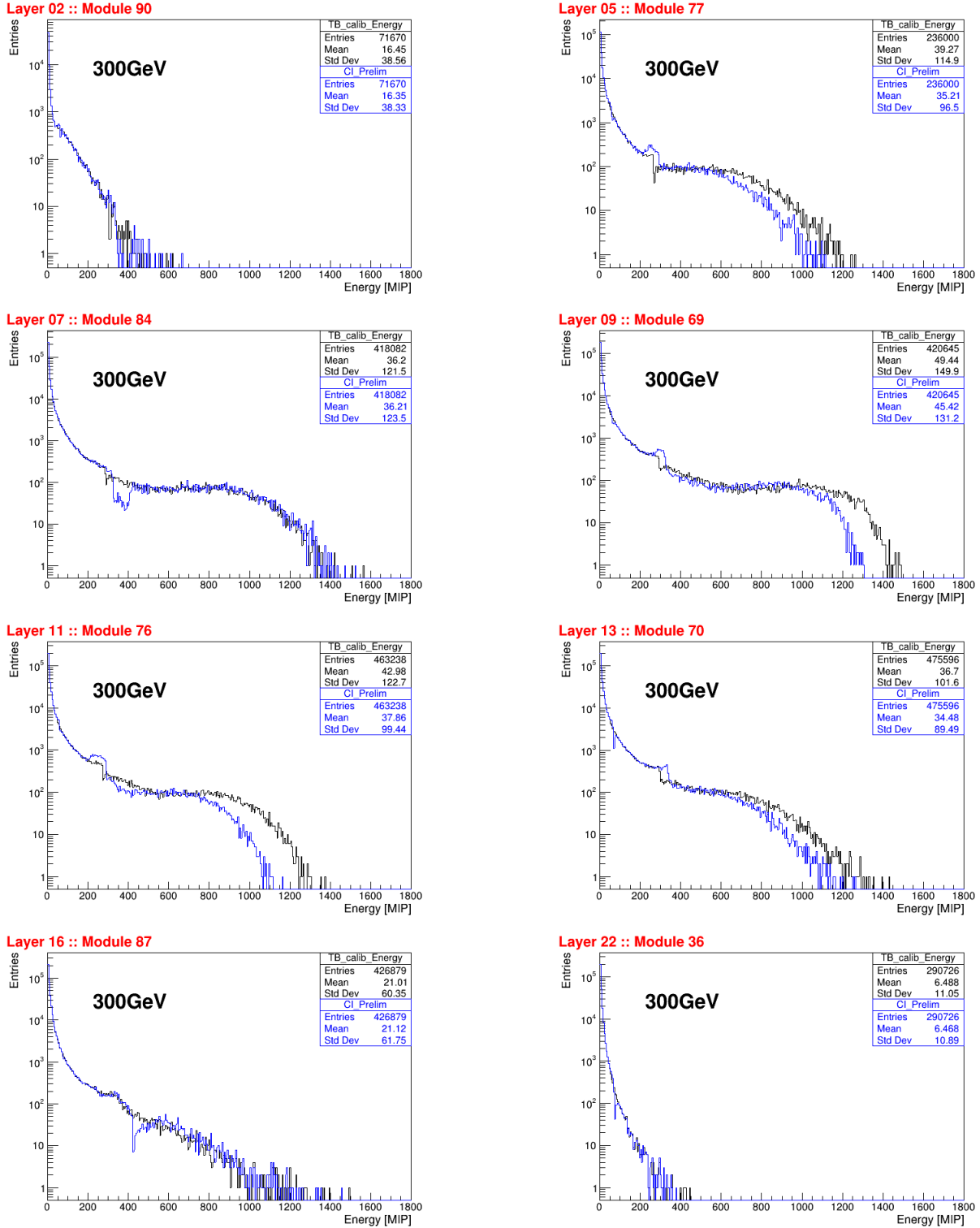
Figure 4.16: Rehit energy spectrum comparison of CI.Prelim with TB_Calib for some layers of CE-E for 300GeV.
