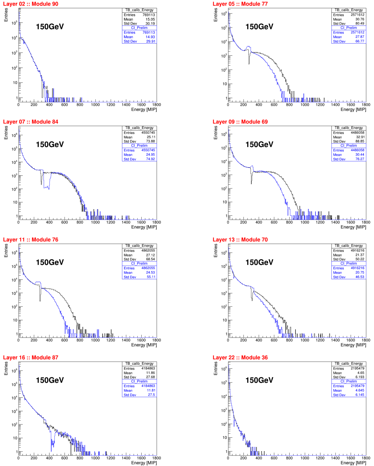
Figure 4.15: Rechit energy spectrum comparison of CI_Prelim with TB_Calib for some layers of CE-E for 150 GeV.
