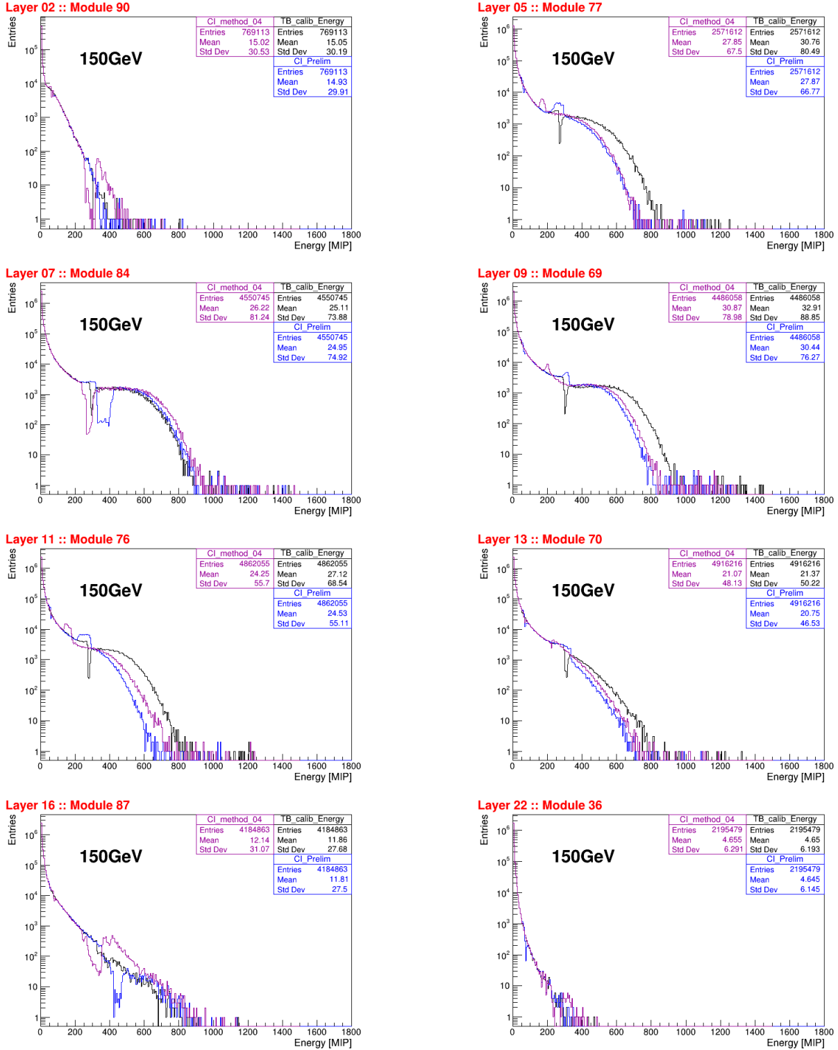
Figure 5.23: Rehit energy spectrum comparison of CI Method 04 with CI_Prelim and TB.Calib for some layers of CE-E for 150GeV.
