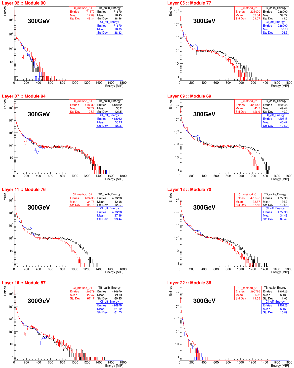
Figure 5.6: Rechit energy spectrum comparison of CI method 01 with CI_Prelim and TB_Calib for some layers of CE-E for 300GeV.
