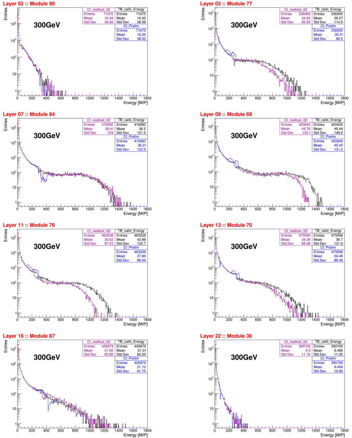
Figure 5.13: Rechet energy spectrum comparison of CI Method 02 with CI.Prelim and TB.Calib for some layers of CE-E for 300GeV.
