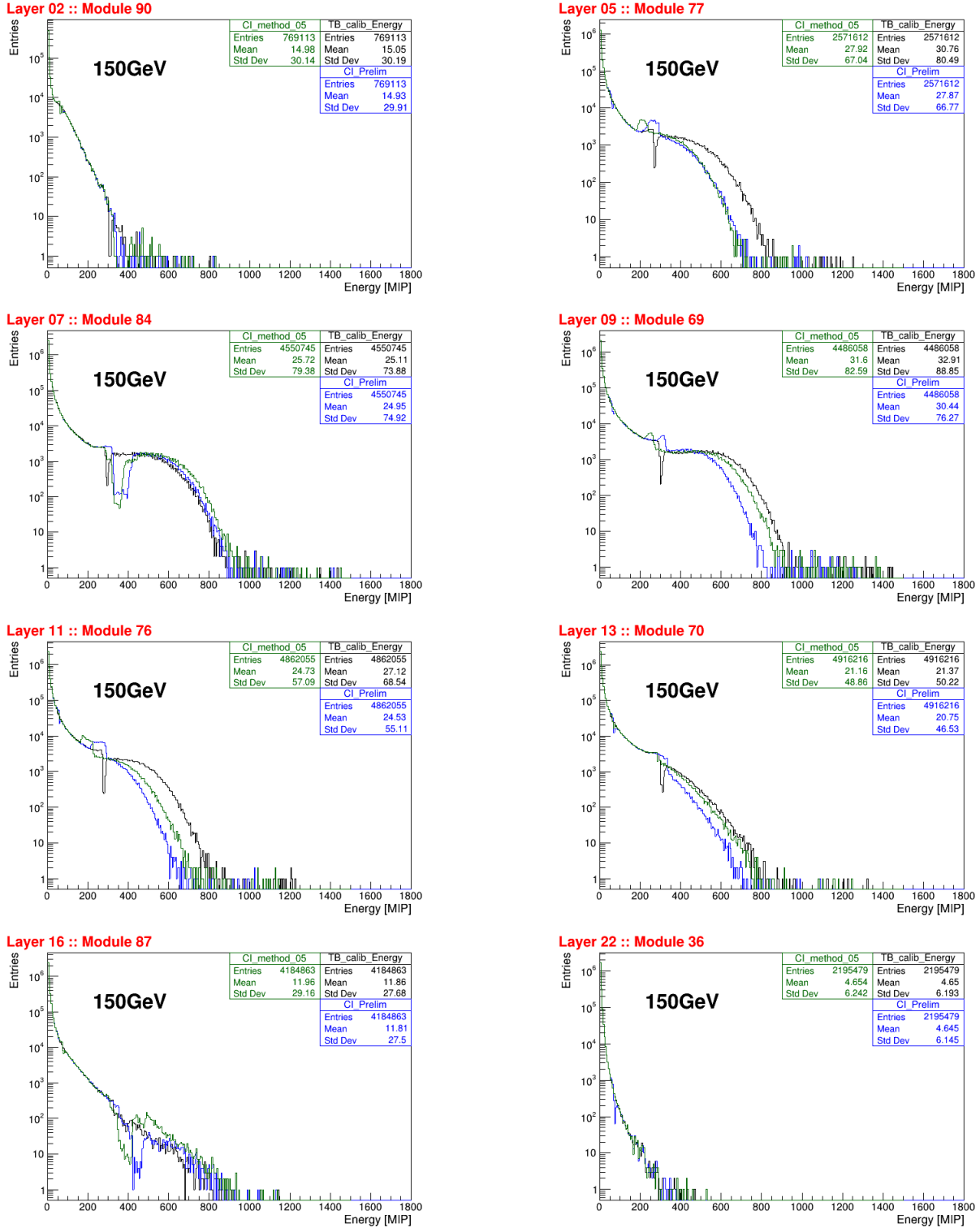
Figure 5.29: Rehit energy spectrum comparison of CI method 05 with CI_Prelim and TB.calib for some layers of CE-E for 150GeV
